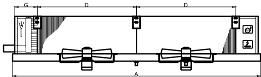
HED/D PLUS 4002/4502/5002/6302/8002
