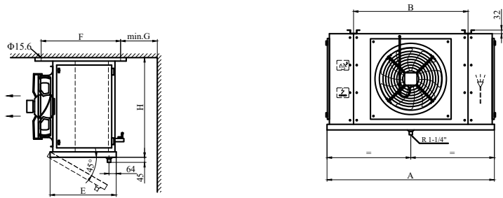
HEB 5501/6301/8001
